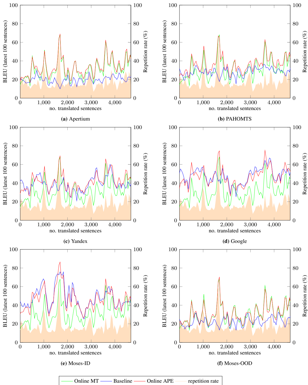
Figure A.11: Dynamics of online learning APE for the EMEA corpus (English to Spanish). The plots show the evolution of BLEU and repetition rate for a window of the latest 100 sentences, as the user completes the translation. The base system is compared to the APE system and a baseline online learning system.
